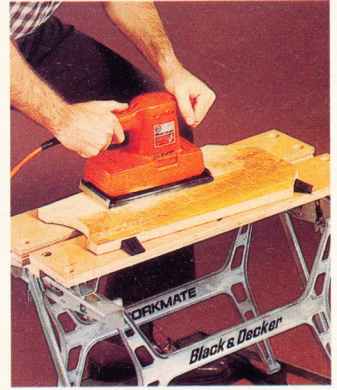
Pegs hold irregular and circular objects
