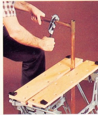
Grooved vise jaws allow vertical grip on pipe and tubing
