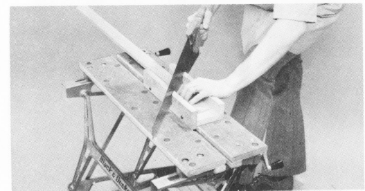
6. Holding a mitre box for more accurate angle cuts. Note: For added rigidity, exert your body weight on the Workmate's base board when sawing or performing other tasks.
