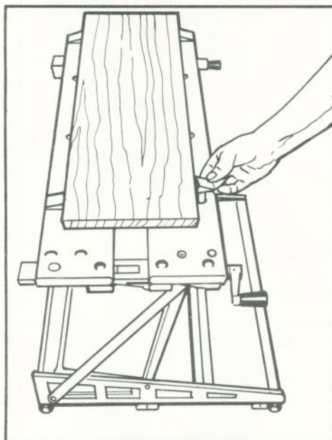
3. Using the vise pegs to extend the vise capacity.
